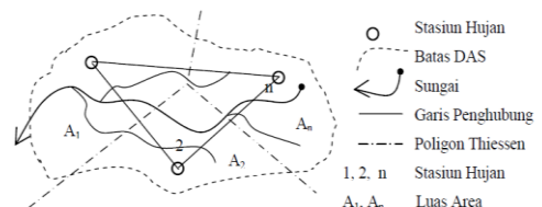
Gambar 2. Metode Thiessen
